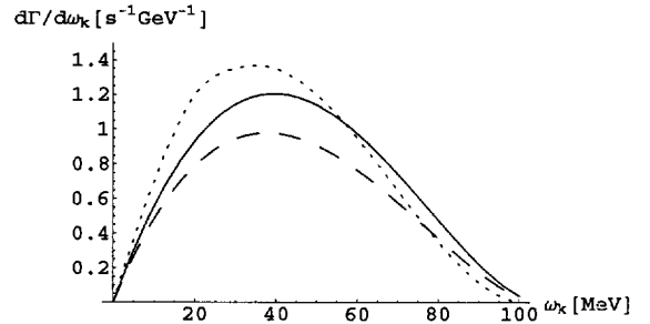
Fig. 7. Spectrum of the emitted photons. The full line represents the full calculation including \mathcal{O}((1/M)^0) and \mathcal{O}((1/M)^1) ; the dashed line represents the result that contains only the \mathcal{O}((1/M)^0) contributions; the dotted line shows the result of [2,5] with g_p = 6.6 g_A .
